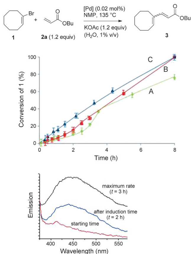
Figure 1. Top graph: Conversion–time plot for the Heck coupling between 1 and 2a with different palladium catalysts in anhydrous media and in the presence of water: A) Pd(OAc) 2 , no water; B) Pd nanoparticles, no water; C) Pd nanoparticles with added water. Bottom graph: Corresponding UV/Vis fluorescence emission spectra (irradiation wavelength: 370 nm) for the anhydrous samples (curves A and B) at different time intervals. Aqueous samples (curve C) gave a similar emission spectrum to that at the maximum rate.
